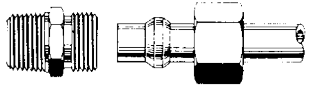
#3RR Male Connector with Roadranger Olive
